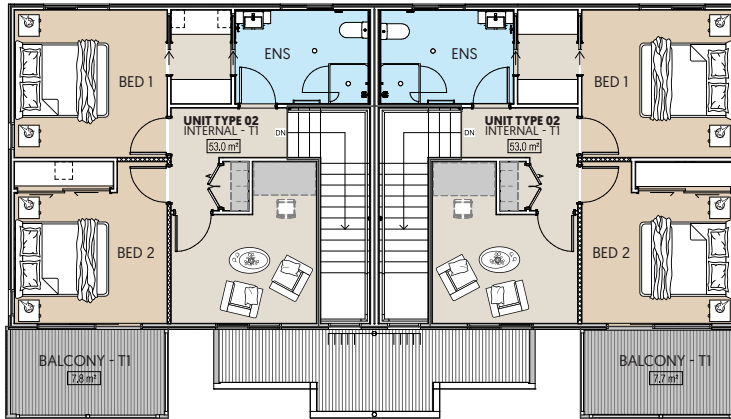
Type B - Floor Plan (Level 2)
