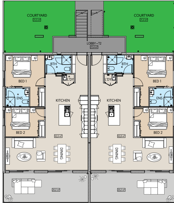
Type A - Level Plan
